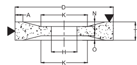
25. Recessed / Relieved & Recessed
