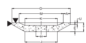
20. Relieved one side
