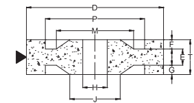
12. Dish
