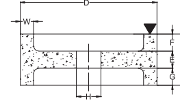
13. Saucer
