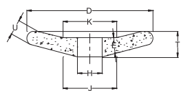
21. Relieved two side
