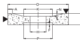
22. Recessed one Relieved other
