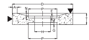
24. Recessed / Relieved & Recessed
