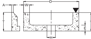
10. Raised dovetail
