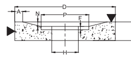
23. Relieved & Recessed Same
